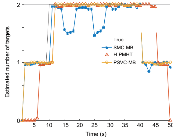
Fig. 8 Estimated number of targets of three different algorithms
