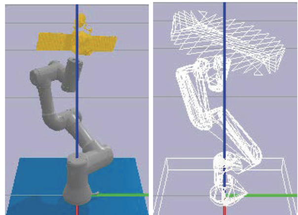
Fig. 3 Virtual environment in PyBullet: visual rendering (left) and collision mesh (right) of the robot model
