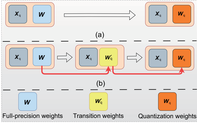
Fig. 2 Illustration of the proposed BDOS: (a) traditional block reconstruction; (b) our proposed BDOS. The description of each parameter is shown in Section 3
