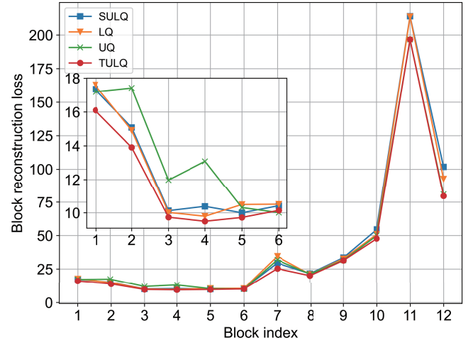
Fig. 5 Comparison of the reconstruction loss in the 12-block 32/3 quantized ViT-S using different quantizers
