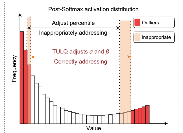
Fig. 1 Illustration of the proposed TULQ
