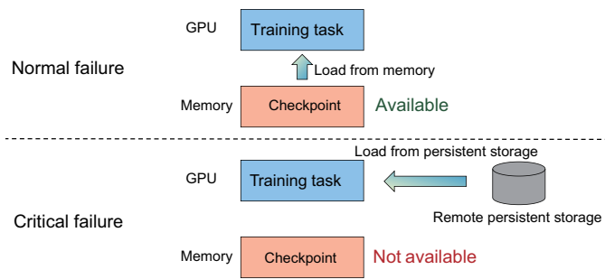
Fig. 2 Difference between the normal failure and critical failure. During normal failures, we load checkpoints from memory; during critical failures, we load checkpoints from remote persistent storage because the checkpoint in memory is not available
