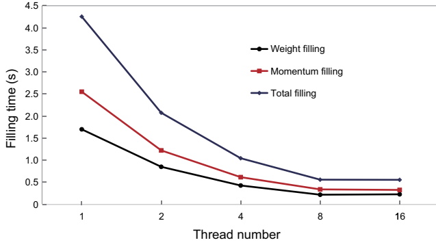
Fig. 19 FastCheck's filling time for different numbers of threads
