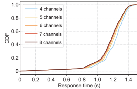
Fig. 3 Cumulative distribution function (CDF) of response time under more channels
