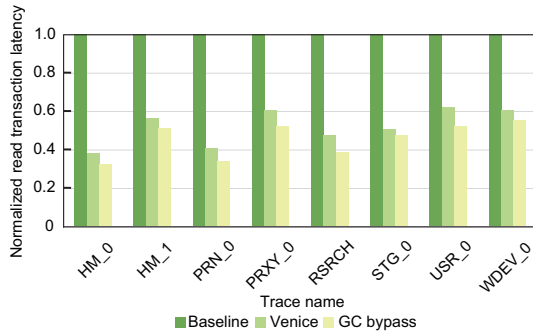
Fig. 9 Normalized read transaction latency
