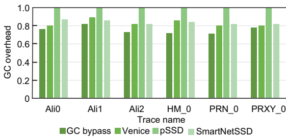
Fig. 16 GC overhead
