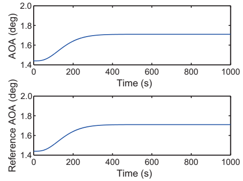
Fig. 6 AOA tracking
