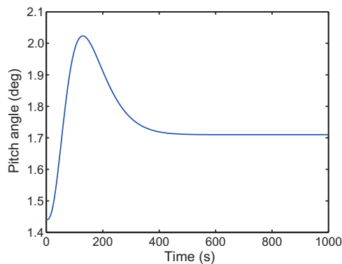
Fig. 9 Pitch angle
