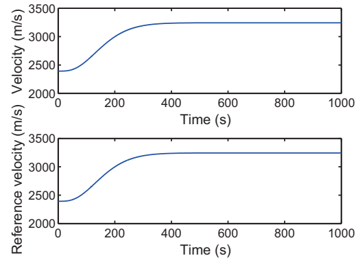
Fig. 2 Velocity tracking
