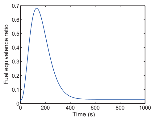
Fig. 11 Fuel equivalence ratio
