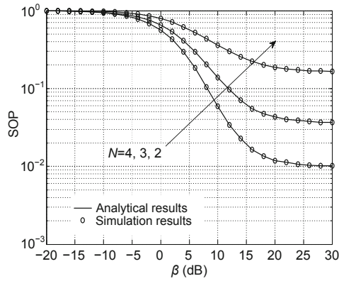
Fig. 1 SOP vs. \beta for various N
