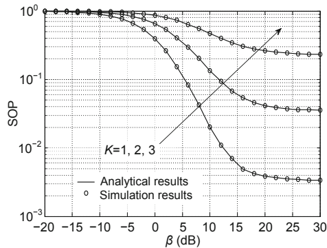
Fig. 2 SOP vs. \beta for various K
