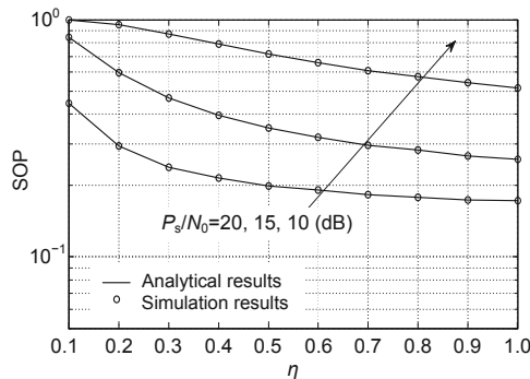
Fig. 5 SOP vs. \eta for various P_s/N_0
