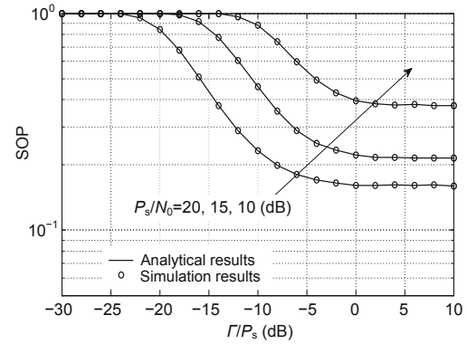
Fig. 3 SOP vs. \Gamma/P_s for various P_s/N_0
