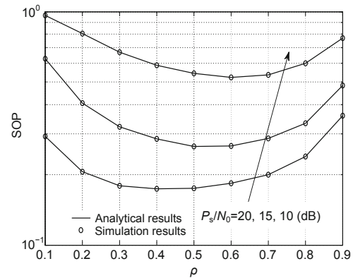
Fig. 4 SOP vs. \rho for various P_s/N_0
