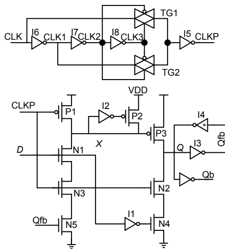
Fig. 5 Conditional discharge flip-flop circuit (Zhao et al., 2004)
