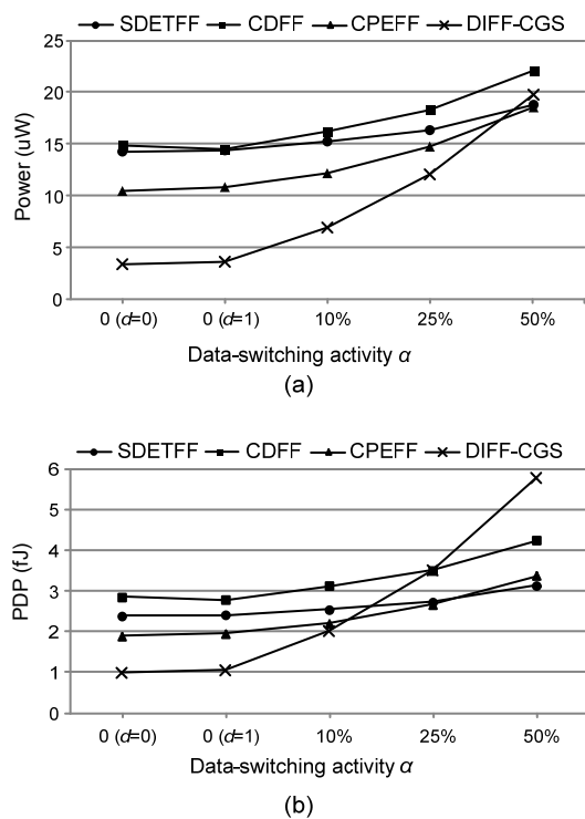
Fig. 12 Different data-switching activities: (a) power dissipation; (b) PDP performance
