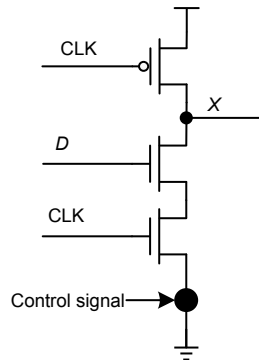
Fig. 4 Conditional discharge technique
