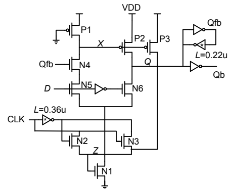
Fig. 6 Conditional pulse-enhancement flip-flop circuit (Hwang et al., 2012)
