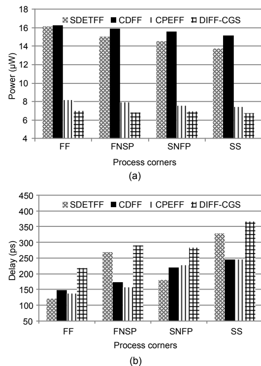
Fig. 13 Different process corners: (a) power dissipation; (b) delay
