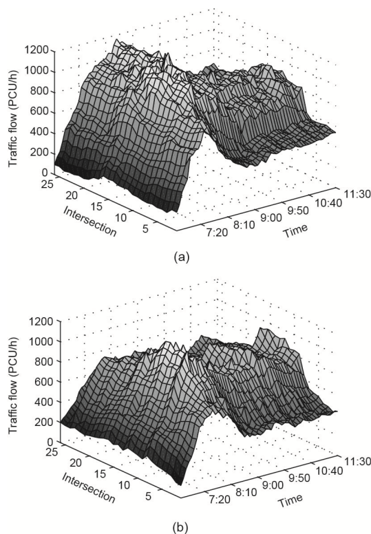
Fig. 10 The going straight traffic flow of Zhongxing Road on January 20, 2016: (a) south to north; (b) north to south
