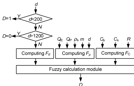
Fig. 3 Flowchart of the degree of correlation calculation
