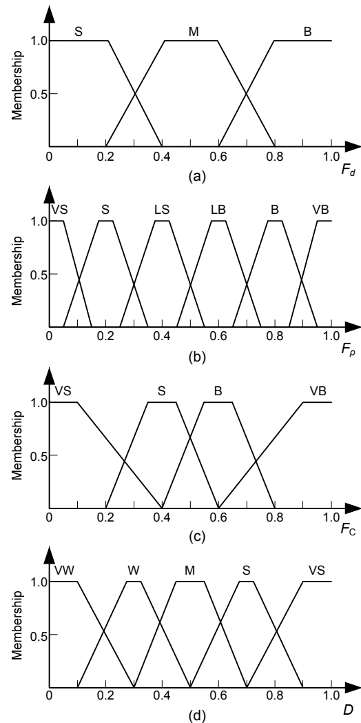
Fig. 4 The membership of fuzzy sets: (a) fuzzy sets defined on F_d ; (b) fuzzy sets defined on F_\rho ; (c) fuzzy sets defined on F_C ; (d) fuzzy sets defined on D
