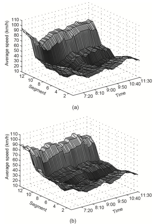
Fig. 11 The going straight average speed of vehicles on Zhongxing Road on January 20, 2016: (a) south to north; (b) north to south
