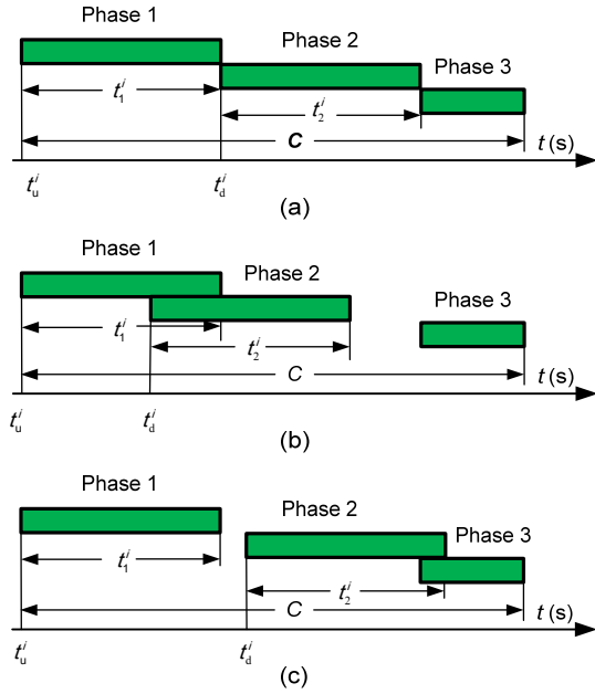
Fig. 6 Three possible configurations of the phase time series: (a) connection; (b) overlap; (c) separation
