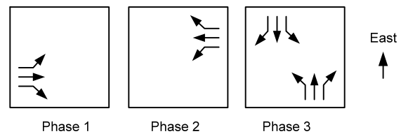
Fig. 5 Initial phase configuration
