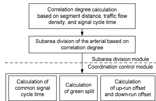
Fig. 2 Framework for the coordination control method
