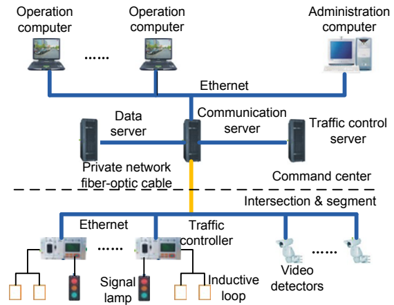
Fig. 8 Architecture of the dynamic traffic coordination control system
