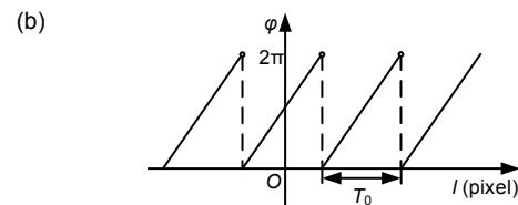
Fig. 3 Phase estimation (a) and the phase variation with the displacement of the moiré fringe (b)
