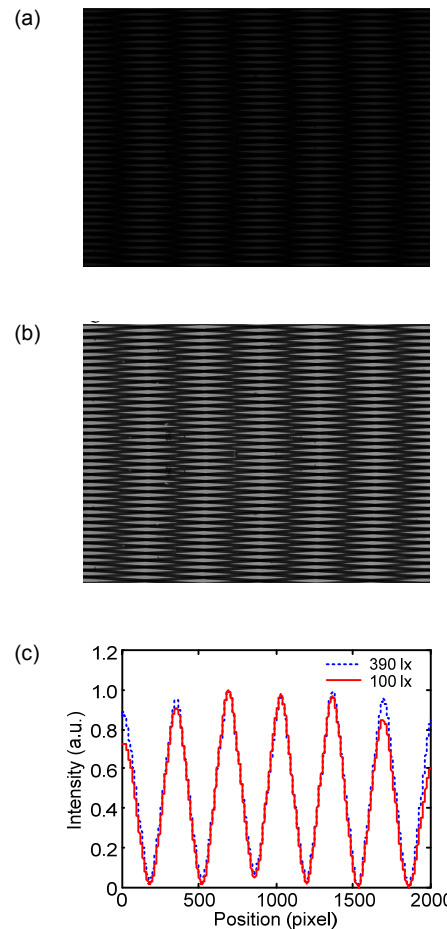
Fig. 5 Digital moiré fringes obtained at 100 lx (a) and 390 lx (b), respectively, and the corresponding digital moiré curves (c)
