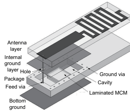
Fig. 11 Expanded view of the proposed system
