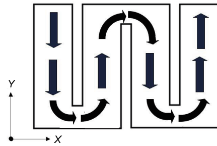
Fig. 2 Direction of current in the meander line antenna
