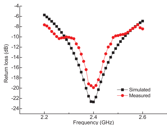
Fig. 13 Measured and simulated return loss characteristics
