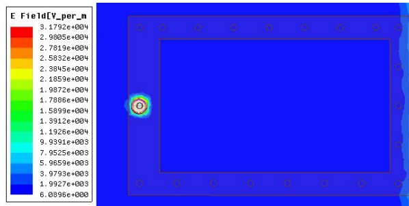
Fig. 10 Electric field intensity of the packaging layer. References to color refer to the online version of this figure
