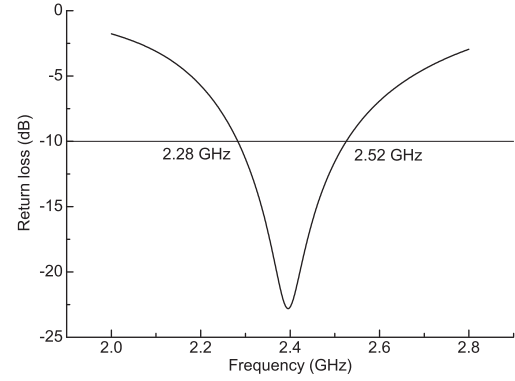
Fig. 3 Simulated return loss characteristics of the proposed antenna
