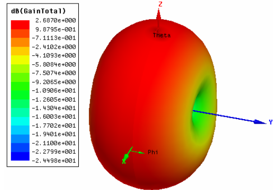
Fig. 5 Simulated 3D radiation pattern at 2.4 GHz. Reference to color refer to the online version of this figure
