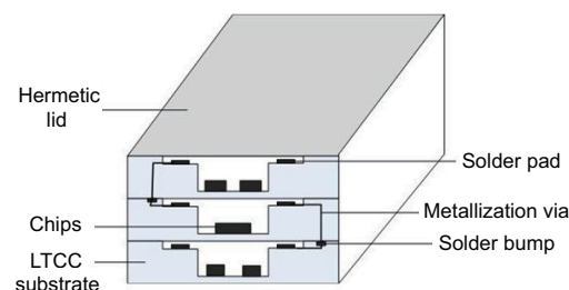
Fig. 8 Illustration of the laminated LTCC MCM
