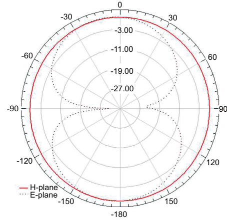
Fig. 4 Simulated E- and H-plane radiation patterns at 2.4 GHz
