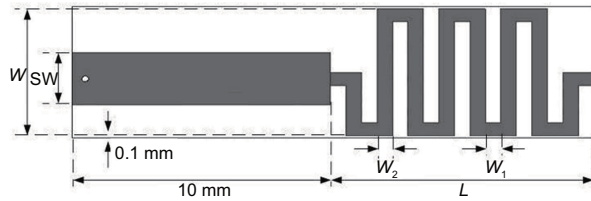
Fig. 1 Design parameters of the meander line antenna
