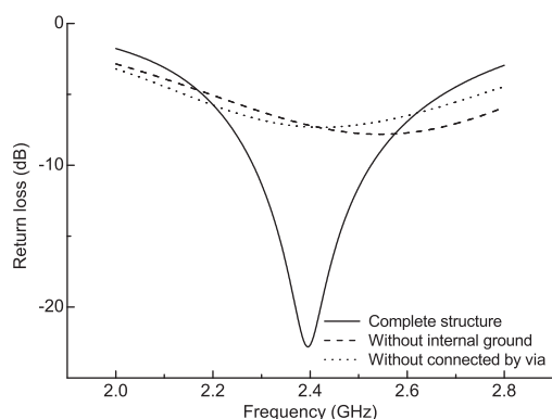
Fig. 6 Return loss characteristic of different internal ground configurations
