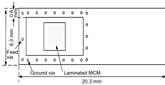
Fig. 9 Design parameters of the packaging layer
