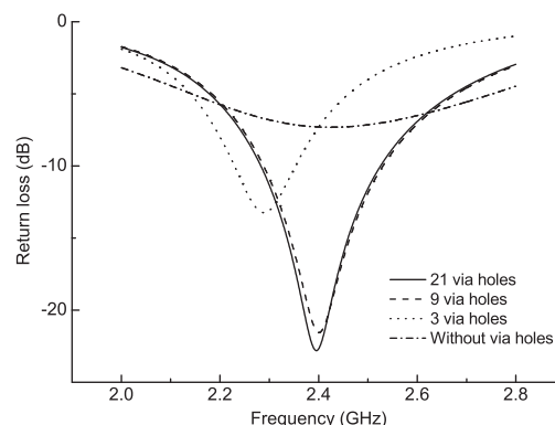
Fig. 7 Return loss characteristic of the various number of via holes
