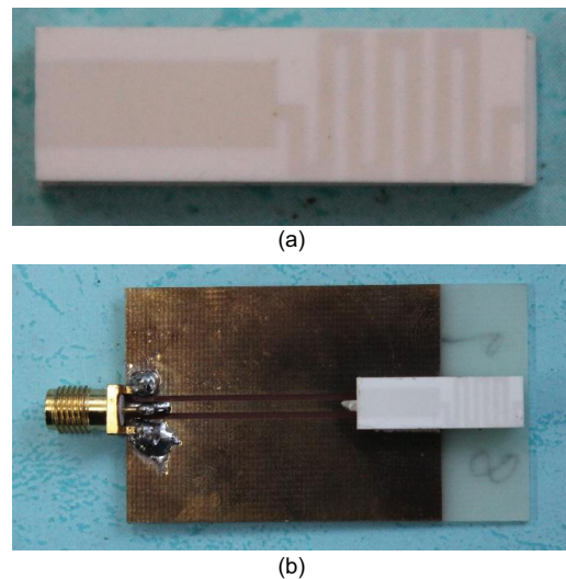
Fig. 12 Fabricated AiP system (a) and testing environment (b)
