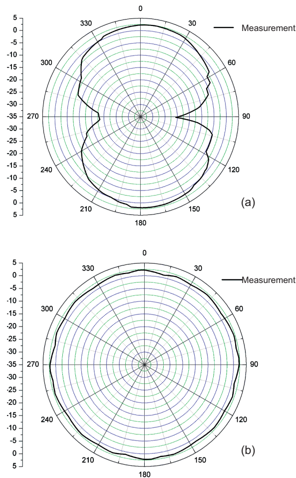
Fig. 14 Measured E-plane radiation pattern (a) and H-plane radiation pattern (b)
