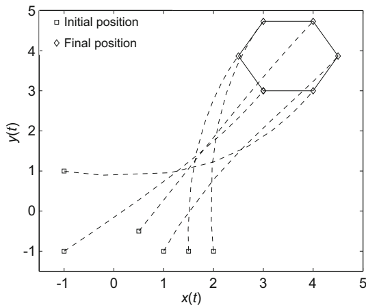
Fig. 7 Formation for the six agents (Example 3)
