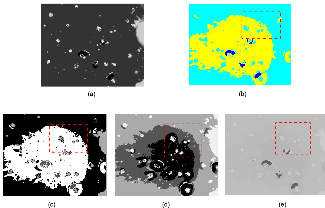
Fig. 13 Comparison of the segmentation results of the proposed algorithm and four state-of-the-art segmentation algorithms: (a) image segmentation object in this study; (b) FCM_S segmentation result; (c) FLICM segmentation result; (d) DSFCM segmentation result; (e) FRFCM segmentation result (References to color refer to the online version of this figure)
