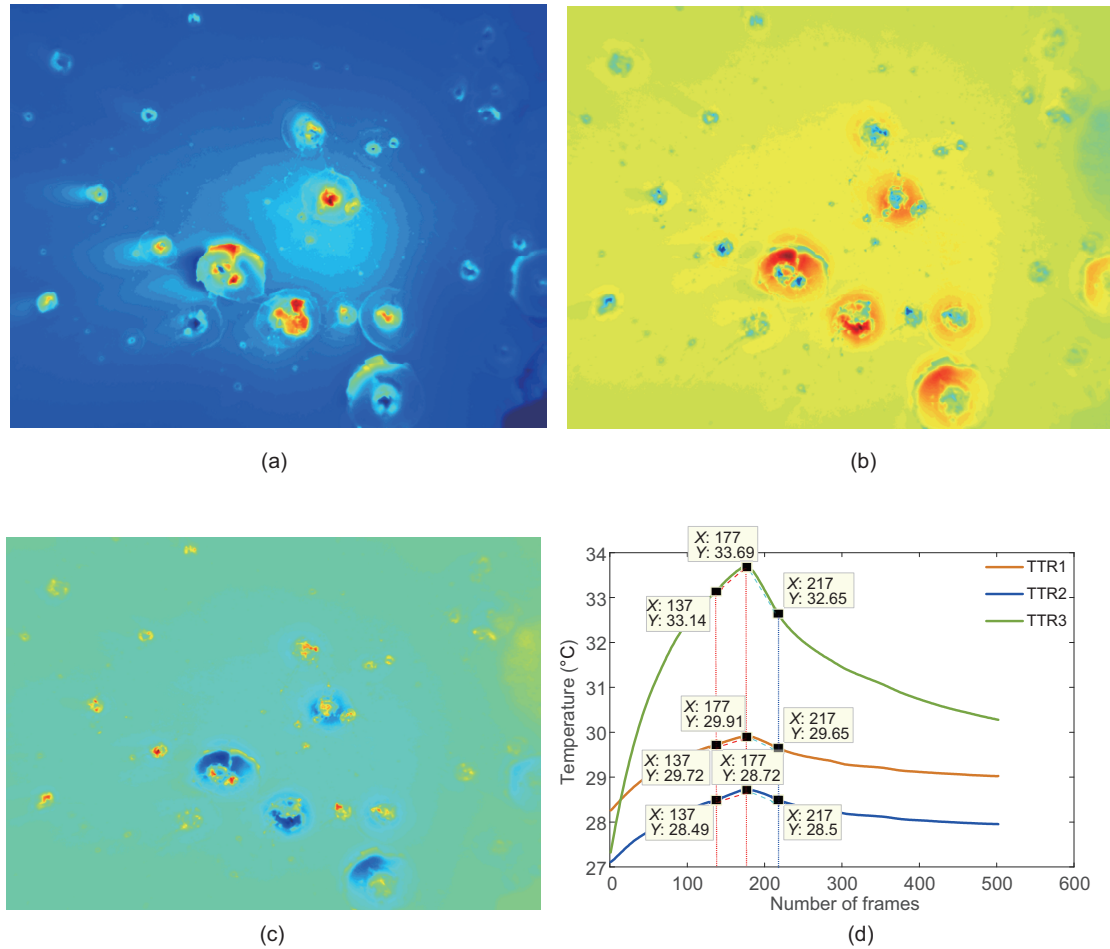
Fig. 9 IRRI acquisition results for the sample: (a) stress damage around the perforation defect; (b) drum kit; (c) perforation damage; (d) TTR for damage (References to color refer to the online version of this figure)
