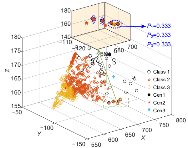
Fig. 7 FCM classification results for the sample (References to color refer to the online version of this figure)
