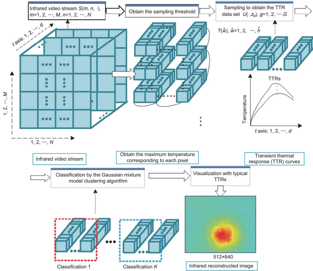
Fig. 5 Schematic of infrared reconstructed image (IRRI) generation
