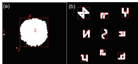
Fig. 12 Segmentation marking results of damage characteristic regions of samples A (a) and B (b)
