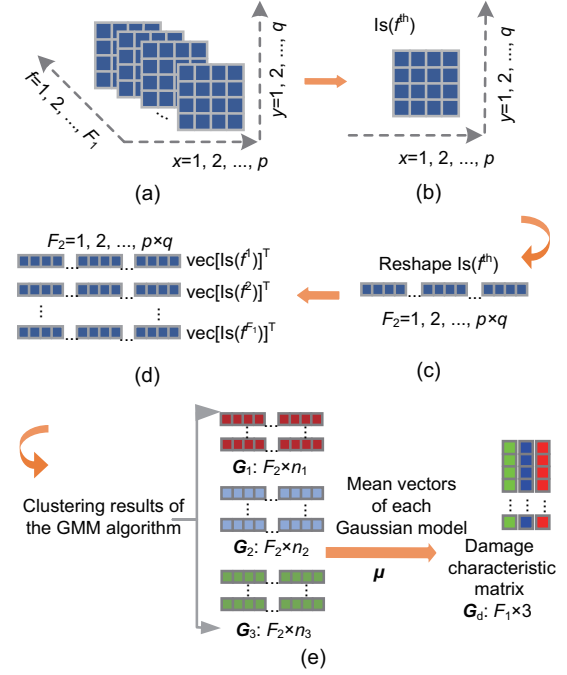
Fig. 2 Schematic of the data conversion and clustering: (a) image sequence Is(f) ; (b) f^{th} frame of Is(f) ; (c) vec[Is(f^{th})]^T ; (d) reconstruction matrix O_{ttr} ; (e) damage characteristic matrix construction
