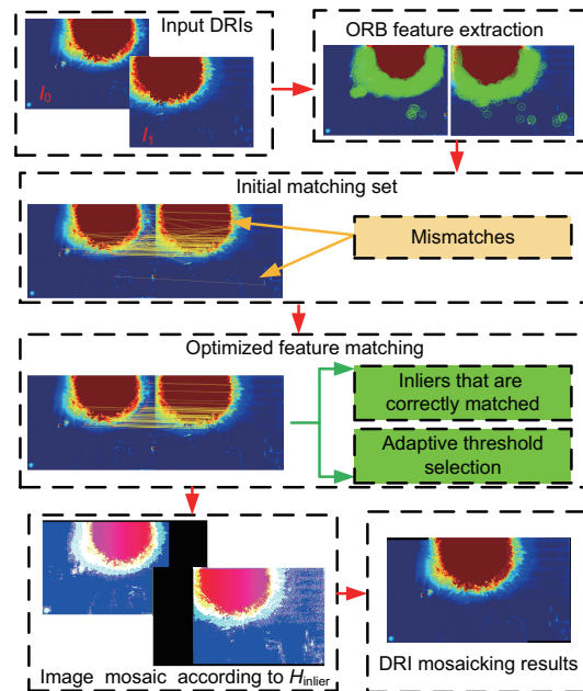
Fig. 4 Schematic of the image mosaicking scheme
