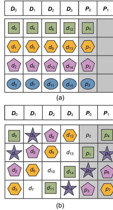
Fig. 5 Encoding of RDP code when k = 4 , m = 2 , and w = 4 : (a) P_0 parity layout; (b) P_1 parity layout
