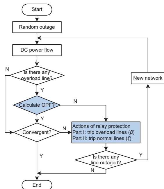
Fig. 1 Inner iteration of the improved ORNL-PSERC-Alaska (OPA) model (DC: direct current; OPF: optimal power flow)
