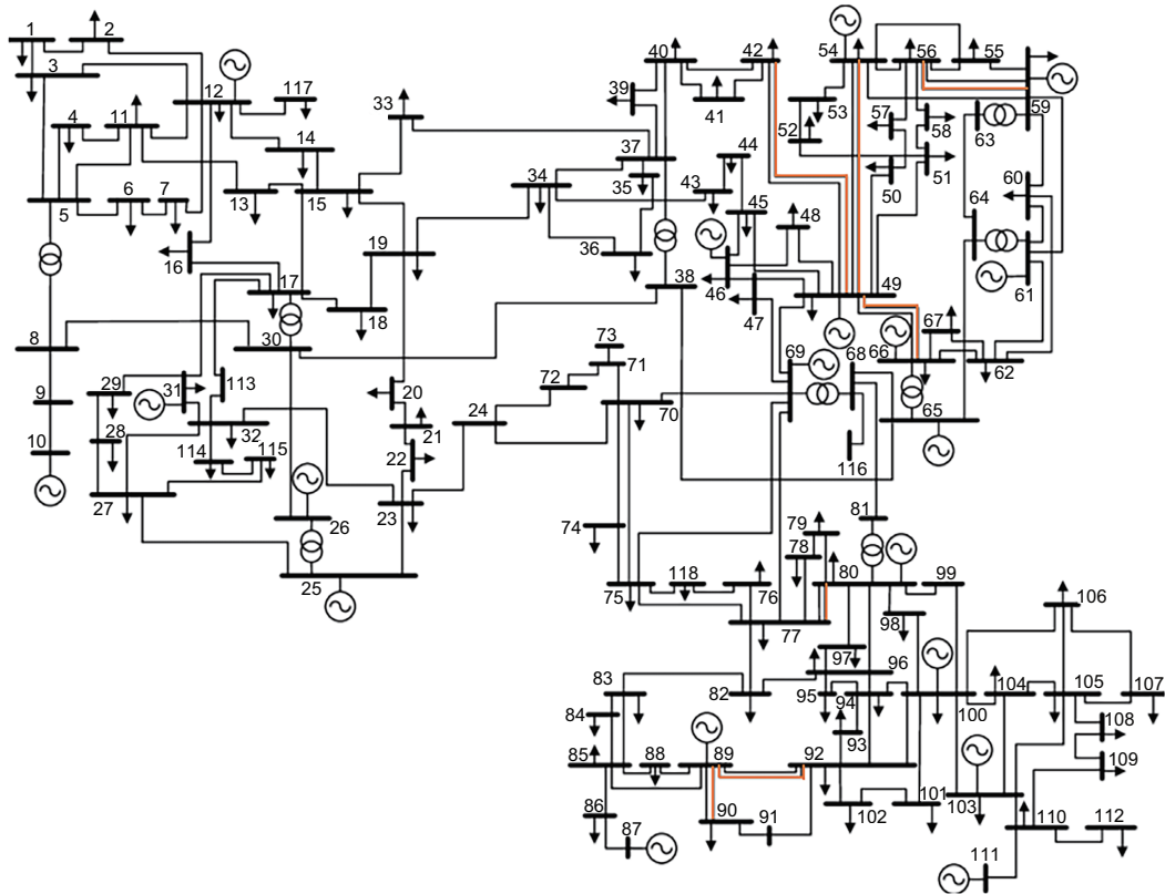
Fig. 5 Topology of IEEE 118 with parallel (double) lines (orange lines represent the redundancy lines). References to color refer to the online version of this figure
