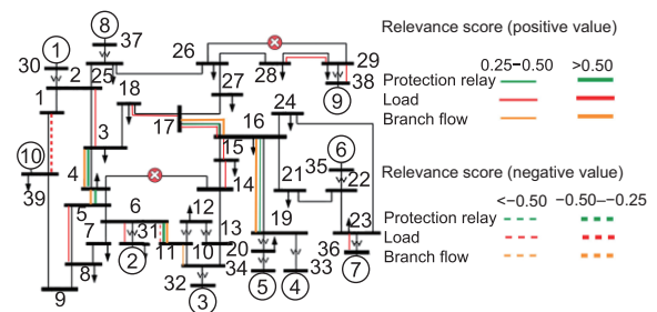
Fig. 10 Topological graph representing a part of IEEE 39 after L9 and L44 are triggered. The target class is predicted as a high-level component outage. References to color refer to the online version of this figure
