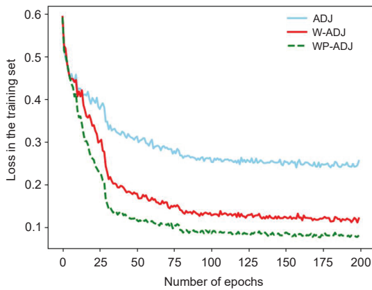
Fig. 7 The curve of loss in the IEEE 39 test system using the MGCN model
