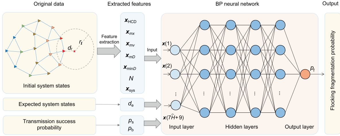
Fig. 5 Neural network architecture for fragmentation problem formulation
