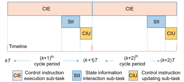
Fig. 1 Illustration of communication-computation-execution cycles
