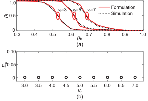
Fig. 10 Coincidence degree (a) and mean square error E_c (b) between simulation and theoretical p_b - p_f curves when v_r is set to different values
