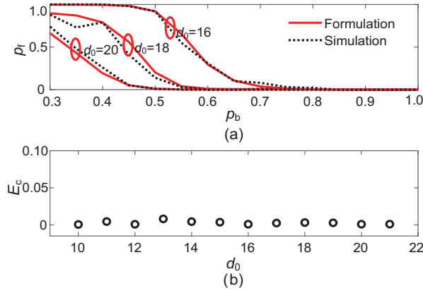
Fig. 8 Coincidence degree (a) and mean square error E_c (b) between simulation and theoretical p_f - p_b curves when d_0 is set to different values
