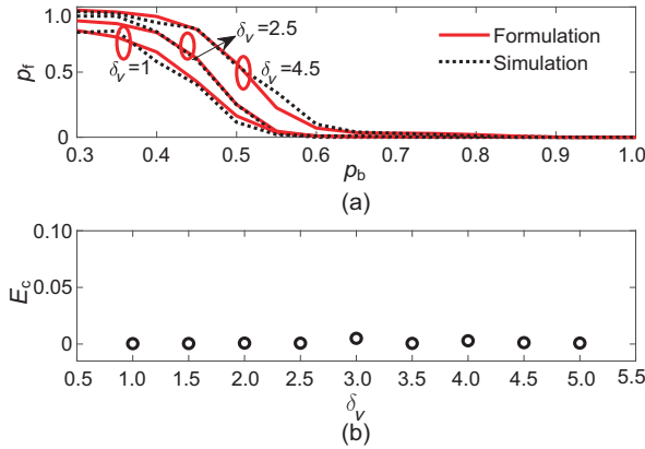
Fig. 7 Coincidence degree (a) and mean square error E_c (b) between simulation and theoretical p_f - p_b curves when \delta_v is set to different values
