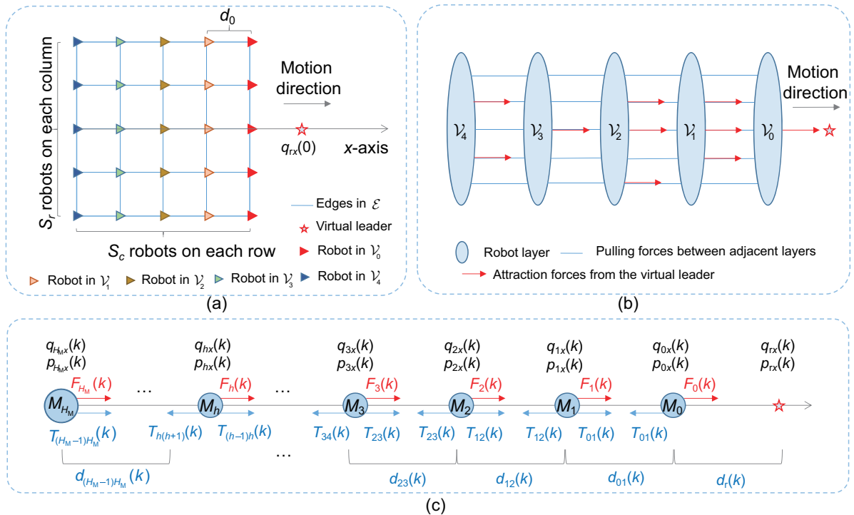
Fig. 3 Initial system states for the simplified flocking scenarios (a), equivalent robot layers and the force illustration of each layer (b), and force illustration for the equivalent centroid points in each layer (c)
