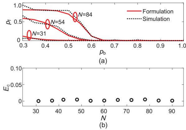
Fig. 6 Coincidence degree (a) and mean square error E_c (b) between simulation and theoretical p_f - p_b curves when N is set to different values
