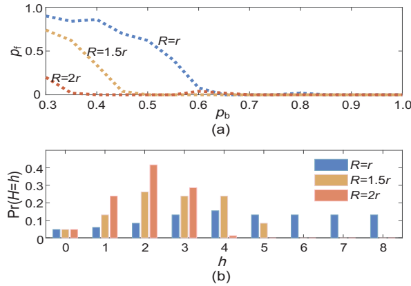
Fig. 11 Illustration of p_b - p_f curves (a) and hop count distribution (b) when LSI's transmission range R is set to r , 1.5r , and 2r
