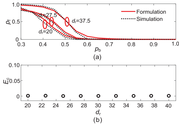
Fig. 9 Coincidence degree (a) and mean square error E_c (b) between simulation and theoretical p_f - p_b curves when d_r is set to different values
