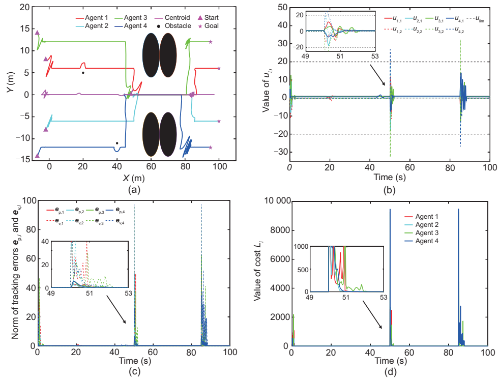
Fig. 7 Control performance of the traditional RLC: (a) trajectories; (b) control inputs; (c) tracking errors; (d) costs (References to color refer to the online version of this figure)
