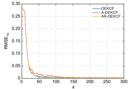
Fig. 9 \text{RMSE}_{\text{TR}} comparison among different algorithms for UAV 2
