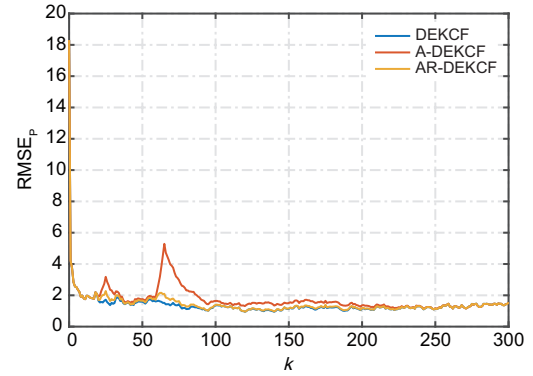
Fig. 7 \text{RMSE}_P comparison among different algorithms for UAV 2
