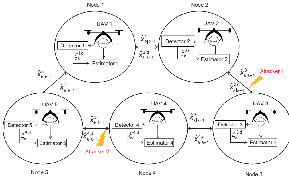
Fig. 2 UAV topology under DALE
