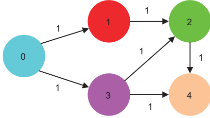
Fig. 6 Communication graph in Examples 1 and 2
