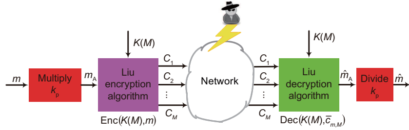
Fig. 3 Block diagram of the improved Liu cryptosystem
